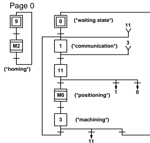
Fig. 2 Page 0 of the Grafcet
