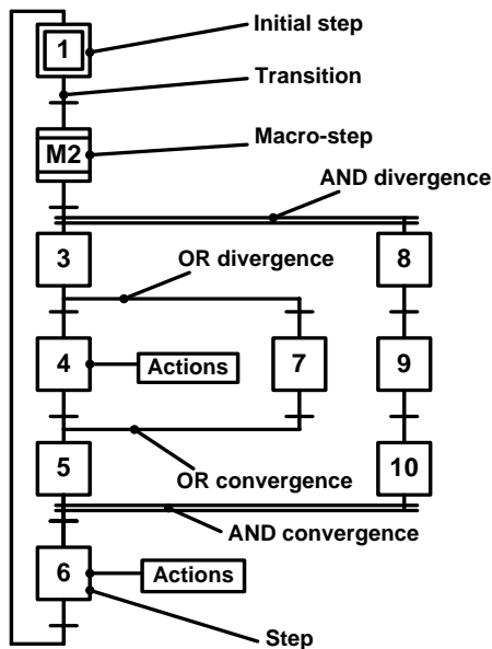
Fig. 1 An example of a Grafset flowchart
