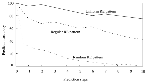
Fig. 10. Average prediction accuracy of MNN
