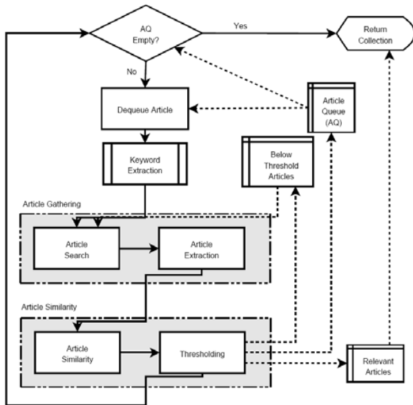
Fig. 1 Overview of proposed method
