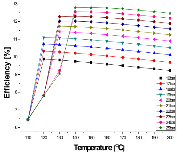
Fig. 9 Cycle efficiency of LT loop with R245fa
