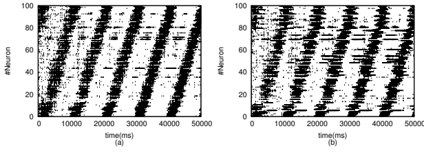
Fig. 7. (a) and (b) Raster plot for different set of fluctuation. (a) (\sigma_{st}, \sigma_{cd}) = (3.0, 1.0) (b) (\sigma_{st}, \sigma_{cd}) = (1.0, 3.0)
