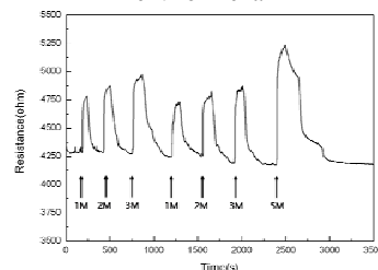
Fig. 6. Resistance changes of the sensor dipped in various methanol concentrations continuously without recovery.
