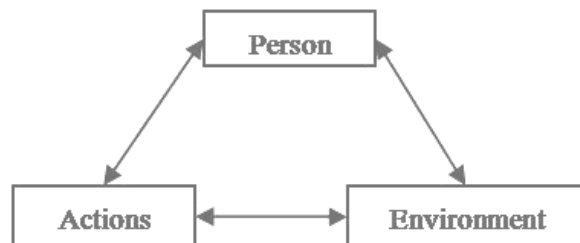
Fig. 1 Judgment framework
