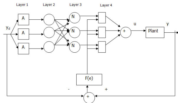
Fig. 1 The Generalized ANFIS Controller
