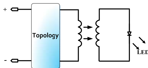
Fig. 1 Typical wireless power transfer system
