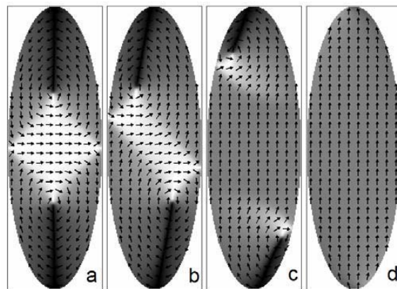
Fig. 4 Magnetization process of a diamond state with lateral dimension 500 \text{ nm} \times 1500 \text{ nm} . (a) shows the demagnetized state in zero field, (b) and (c) show the domain configuration at fields of 13 mT and 19 mT, respectively. In (d) a 25 mT field has been applied.
