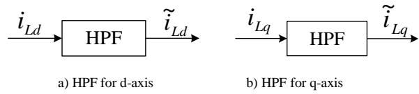
Fig.3 Separation of harmonic components on dq-frame
