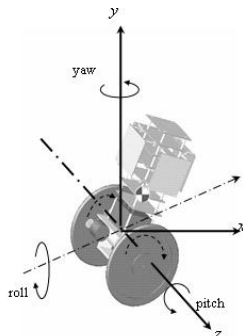
Fig. 1 WIP with its three degree of freedom
