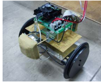
Fig. 3 Wheeled inverted pendulum system
