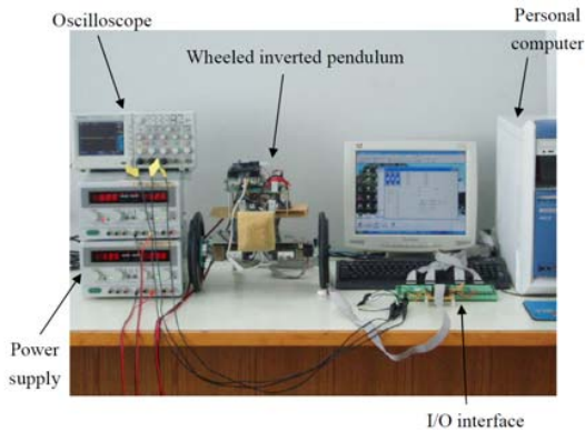
Fig.4 The whole experimental system
