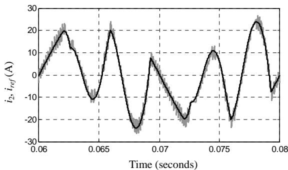
Fig. 8 Waveforms of current to be compensated (in black) and current i_2 (in gray) for L_2=4mH and C_f=0.6\mu F
