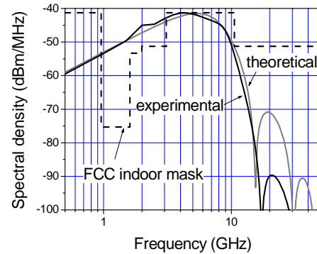
Fig. 3 PSD of the pulse
