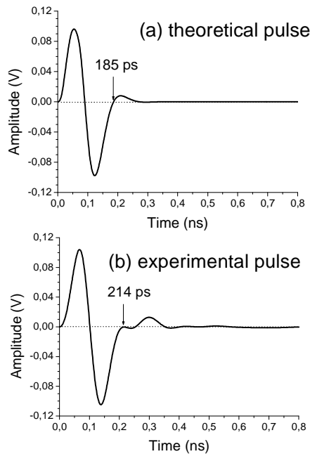
Fig. 2 The generated pulse
