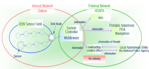
Fig. 3 Intelligent Overload Regulation System
