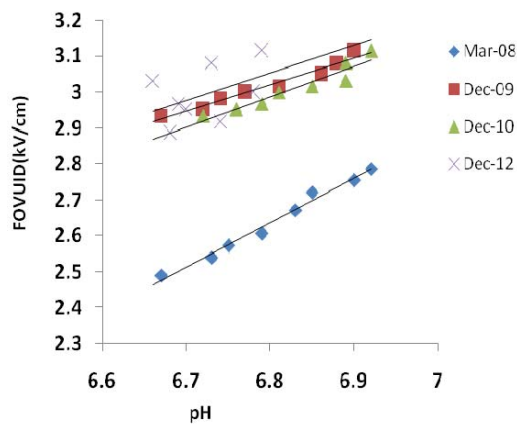
Fig. 5 FOVID vs pH for Location B (Highway)
