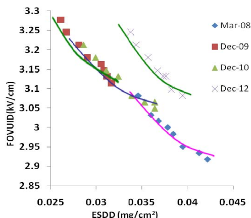
Fig. 1 FOVUID vs ESDD for Location A (Residential)
