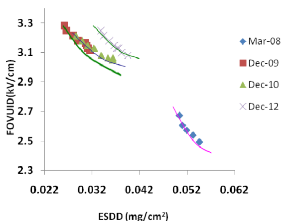
Fig. 2 FOVUID vs ESDD for Location B (Highway)
