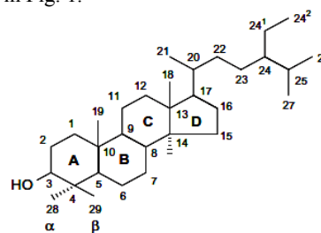
Fig. 1 Basic structure of a sterol with standard carbon numbering according to the IUPAC system
