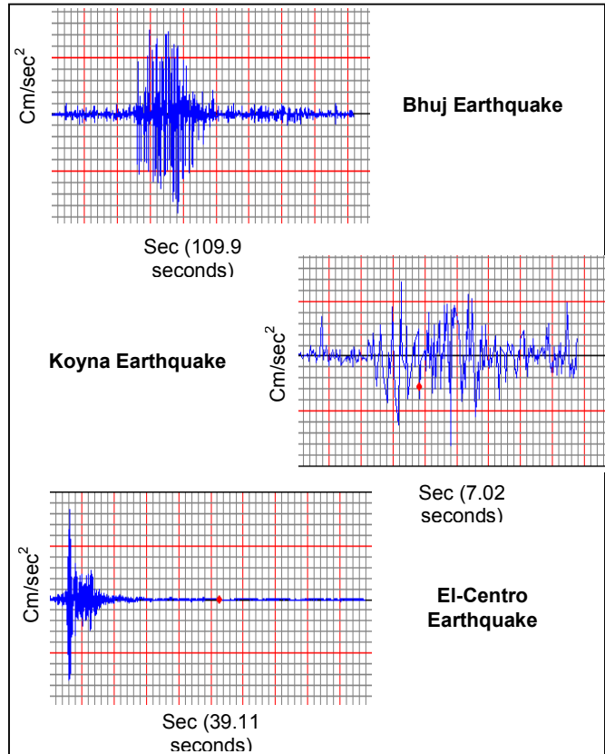
Fig. 8 Time history of earthquake used
