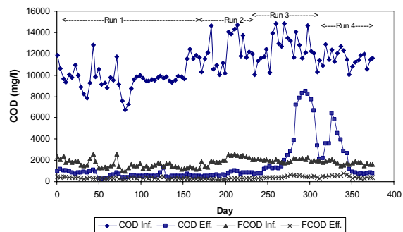
Fig. 2 COD variations
