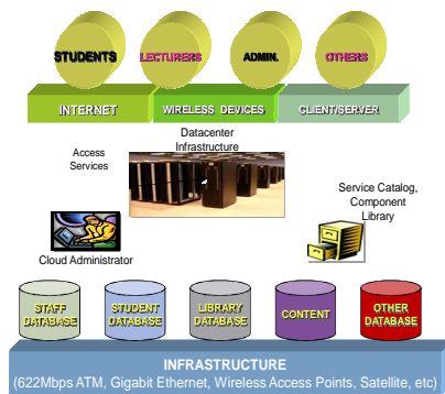
Fig. 4 Proposed Infrastructure Layer in an expandable view
