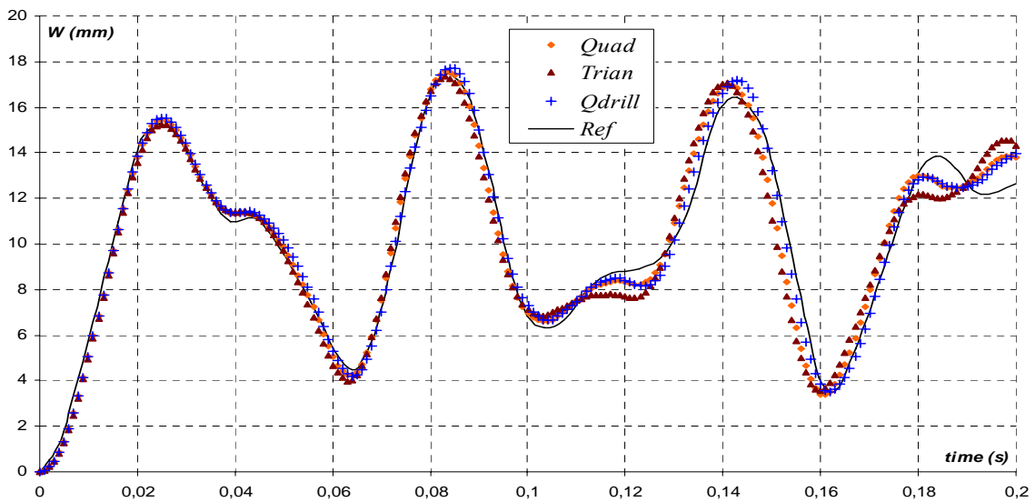
Fig. 6 Vertical displacement time history of the cylindrical shell \alpha=10^{-3}
