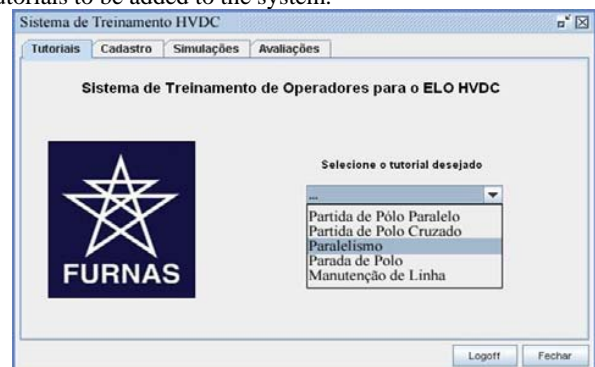
Fig. 11 Selecting tutorial
