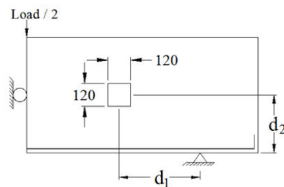
Fig. 13 Square opening
