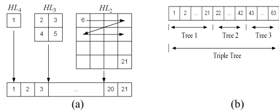
Fig.2 (a) A group of multiwavelet coefficients in each tree and (b) the example of triple tree
