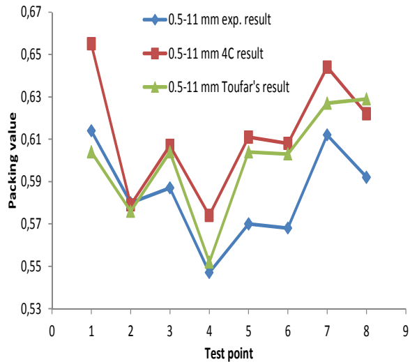
Fig. 7 Representation of the packing results from crushed aggregate 2 tests with packing from 4C program and Toufar model
