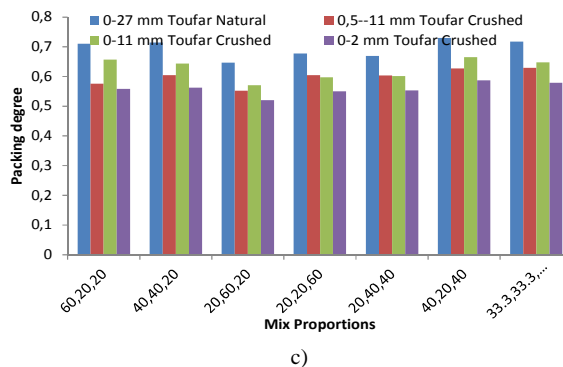
Fig. 13 Comparison between particle packing for natural and crushed aggregate and the same mix proportions, (a) from experimental tests, (b) from 4C program and (c) from Toufar's model
