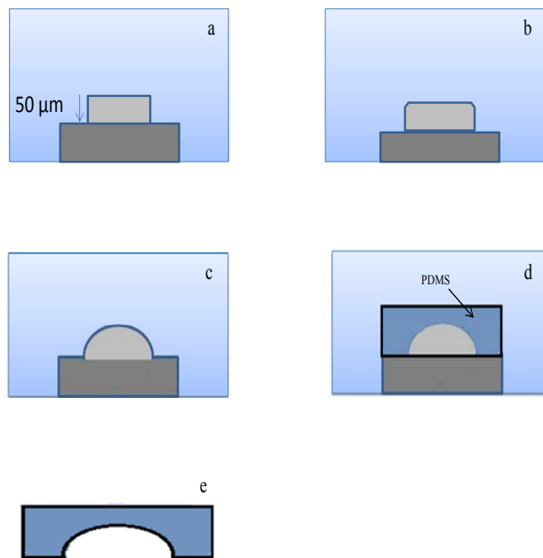
Fig. 5 (a) Structure of mold without heating (b) Structure of mold when photoresist start to change the shape because of reflow at 130^\circ\text{C} for 1 minute (c) Round shape of mold because of reflow at 130^\circ\text{C} for 2 minutes (d) PDMS pouring onto the mold (e) Shape of microfluidic channel after pilling
