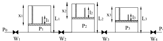
Fig. 1 Three-tank system
