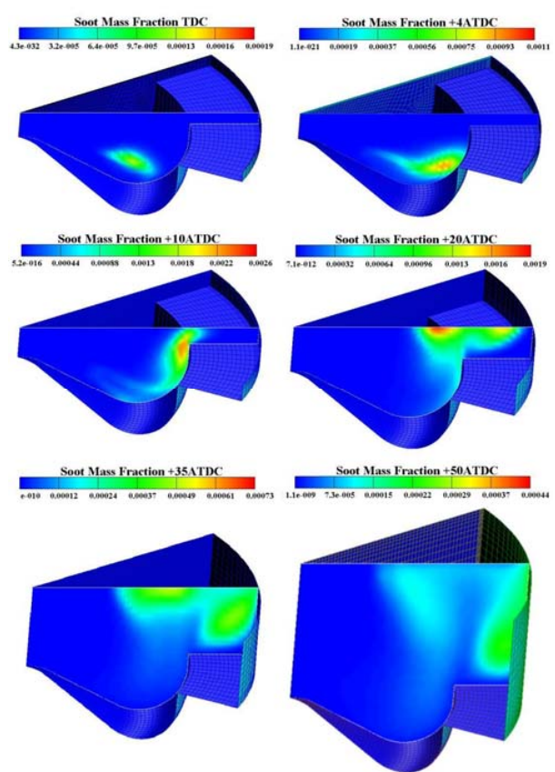
Fig. 7 Predicted soot mass fraction contours at 0, 4, 10, 20, 35, 50 degrees ATDC
