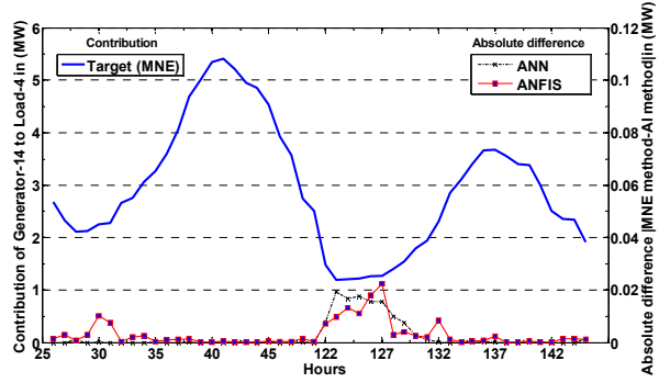
(c) Contribution to load at Bus 4
