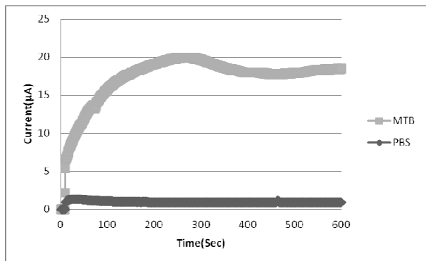
Fig. 2 MTB and PBS buffer comparison
