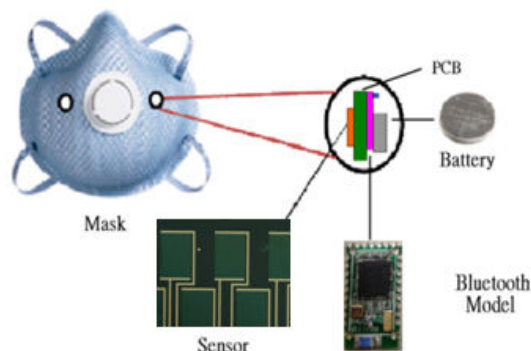
Fig. 10 The schematic equipment of mask-based Lab chip
