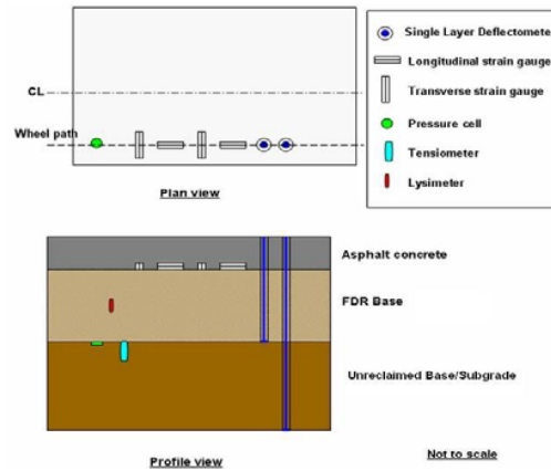
Fig. 5 Pavement Instrumentation
