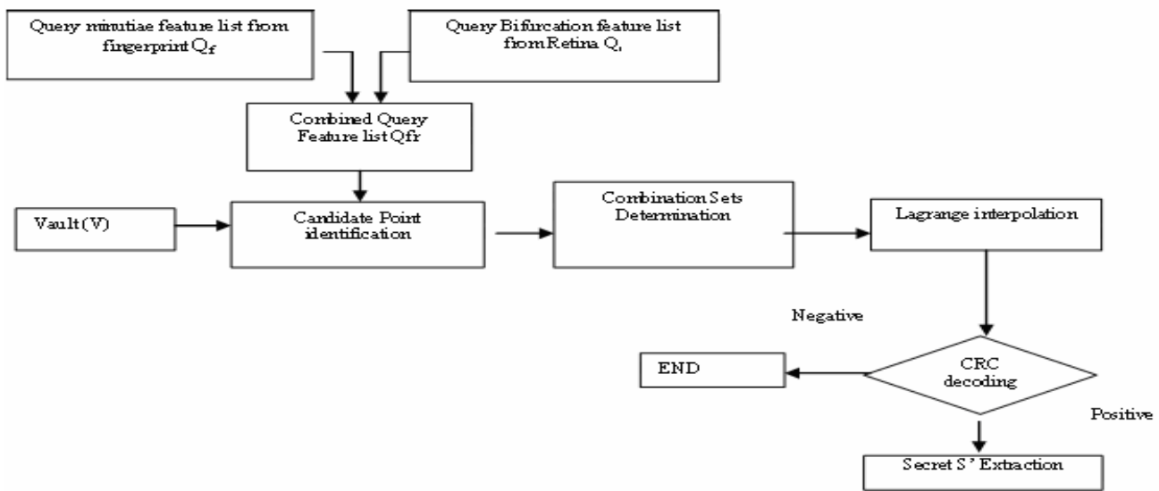
Fig. 5 Multi Biometric Fuzzy Vault: Decoding
