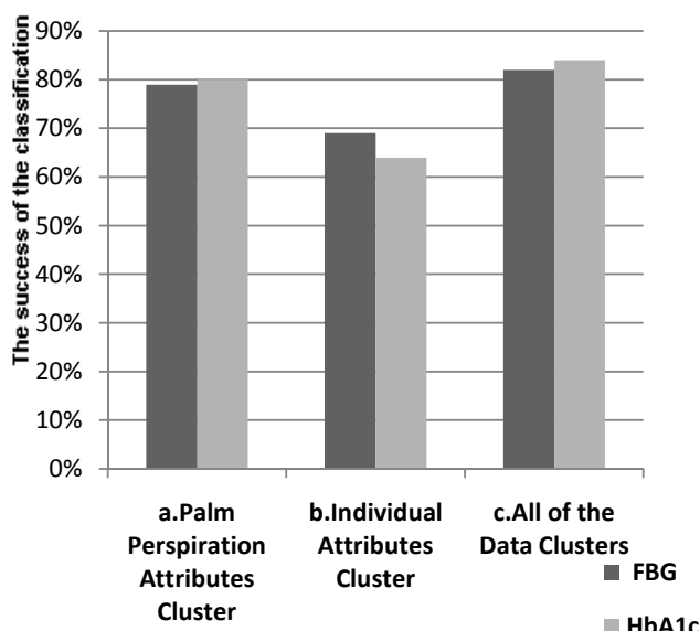
Fig. 6 Results of diabetes diagnosis with SVM
