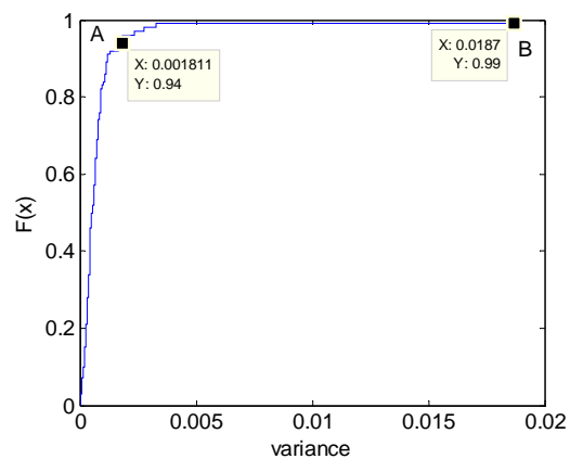
Fig. 5 CDF of variance between AS and DM
