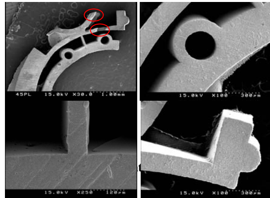
Fig. 6 sintered samples
