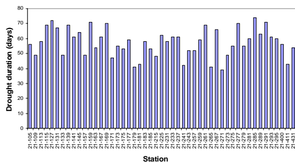
Fig. 4 2-year drought duration of all stations
