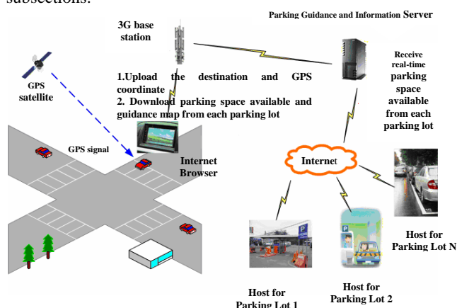
Fig. 2. An integrated architecture of Parking Guidance and Information System
