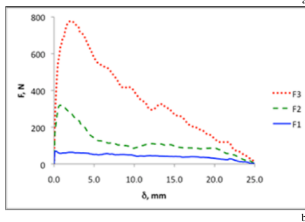
Fig. 1 a) the pull-out specimen's mould; b) pull-out curves ( L = 25 mm, \alpha = 0^\circ ) for: F1 – straight (lower curve); F2 – hooked-end (middle curve); F3 – corrugated (upper curve).
