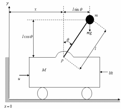
Fig. 1 Inverted pendulum system model
