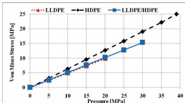
Fig. 4 Variation of Von Mises stress with increasing internal pressure for polymer liner
