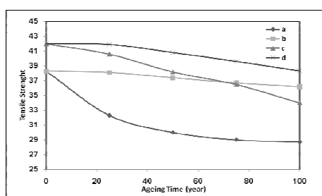
Fig. 2 Tensile strength of (a) uncoated paper, coated paper by (b) ZnO nanoparticles, (c) Klucel, (d) ZnO nanocomposite
