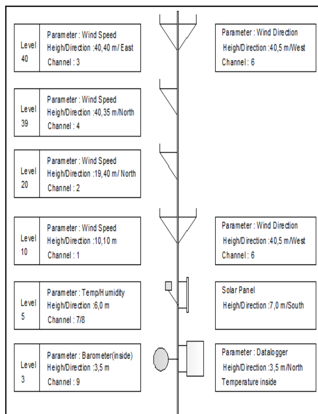
Fig. 1 Meteorological Mast in the El-Maqrun station
