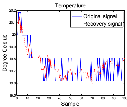
Fig. 11 Comparison of the original signal and the recovery signal of temperature with N = 64
