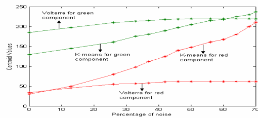
Fig. 5 Noise resistance curve
