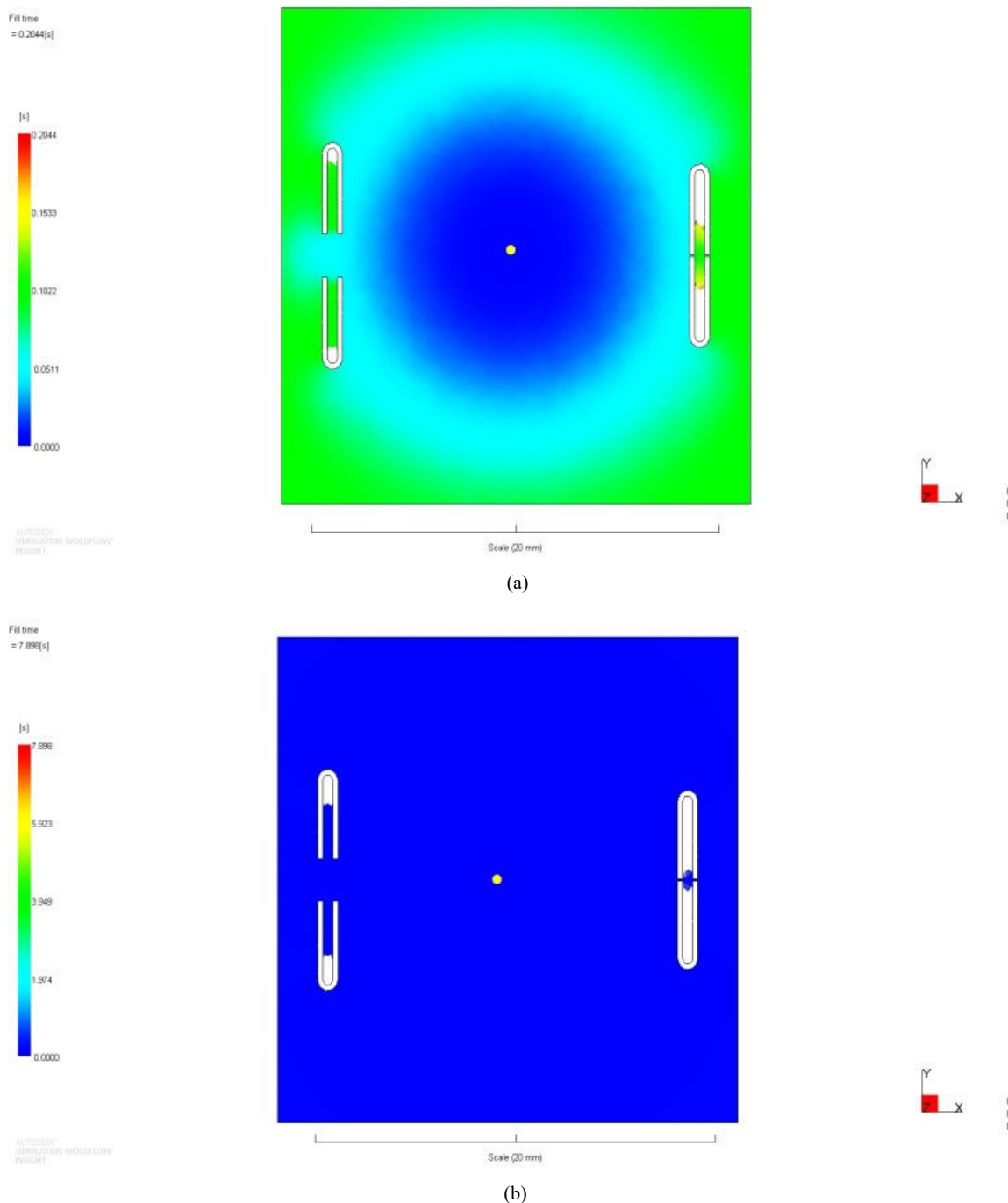
Fig. 7 3D maximum flow length for PP and ABS, (a) R2 and (b) R4
