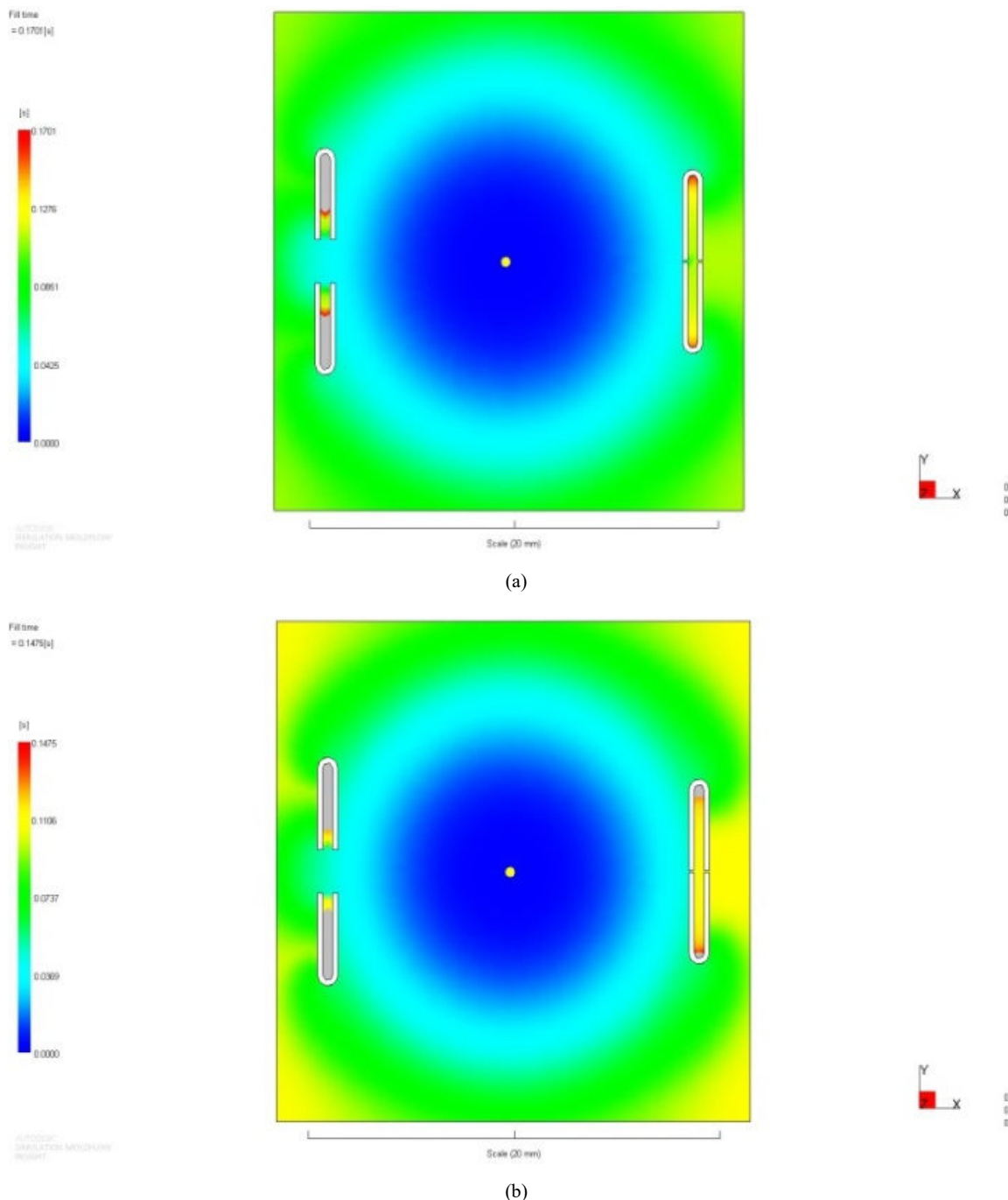
Fig. 5 Dual-domain maximum flow length for PP and ABS, (a) R2 and (b) R4
