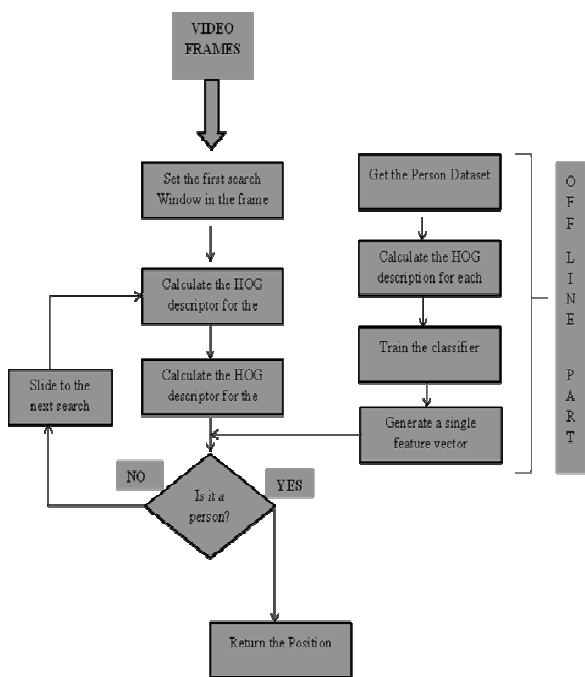
Fig. 1 Person detection system
