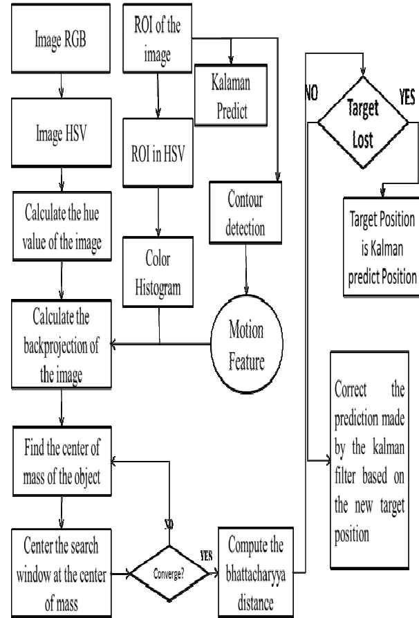
Fig. 3 Flow chart of the tracking system
