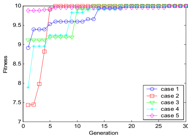
Figure 7 Trace of fitness for five study cases
