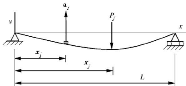
Figure 1 Impact force on a simple supported beam.
