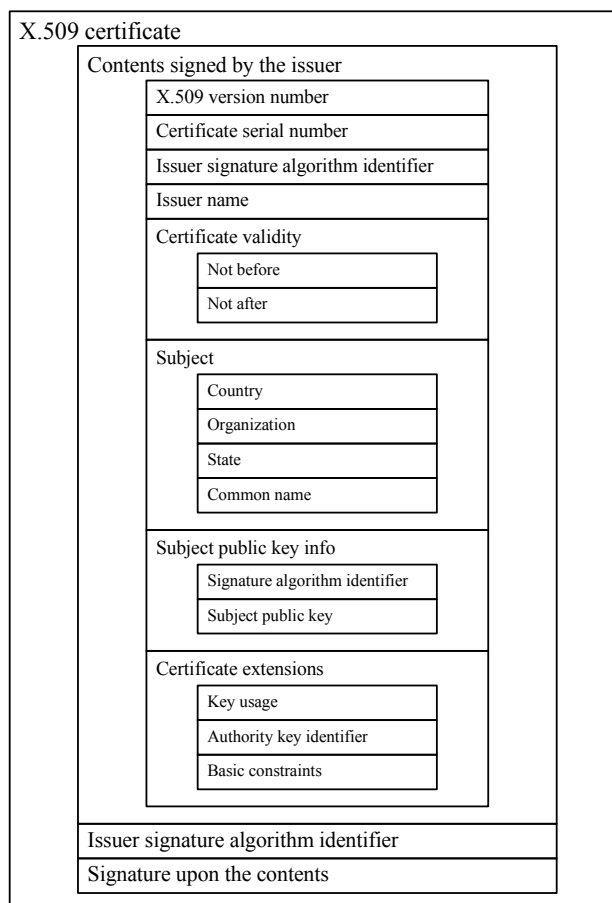
Fig. 1 Structure of an X.509 certificate
