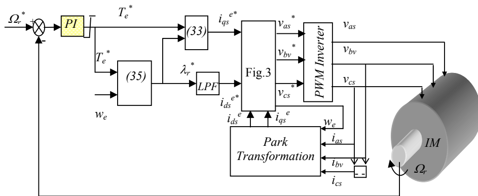
Fig. 5 Configuration system
