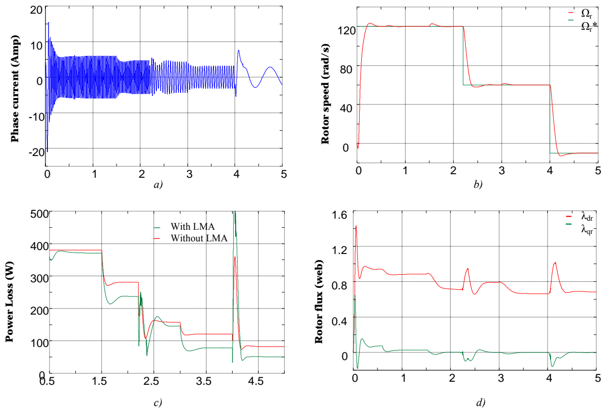
Fig. 7 CaseN o 3: load torque = 10 Nm at starting, T l = 6 Nm at t = 1.5 s, T l = 3 Nm at t = 3 s, Ω r = 120 rad/s at starting, Ω r = 60 rad/s at t = 2.2 s, Ω r = -10 rad/s at t = 4 s
