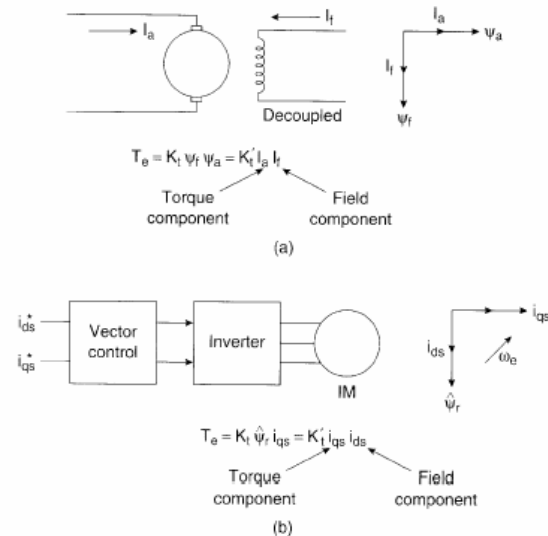
Fig. 1 Principal of field oriented control
