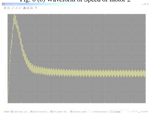
Fig. 6 (c) Waveform of torque of motor 2
